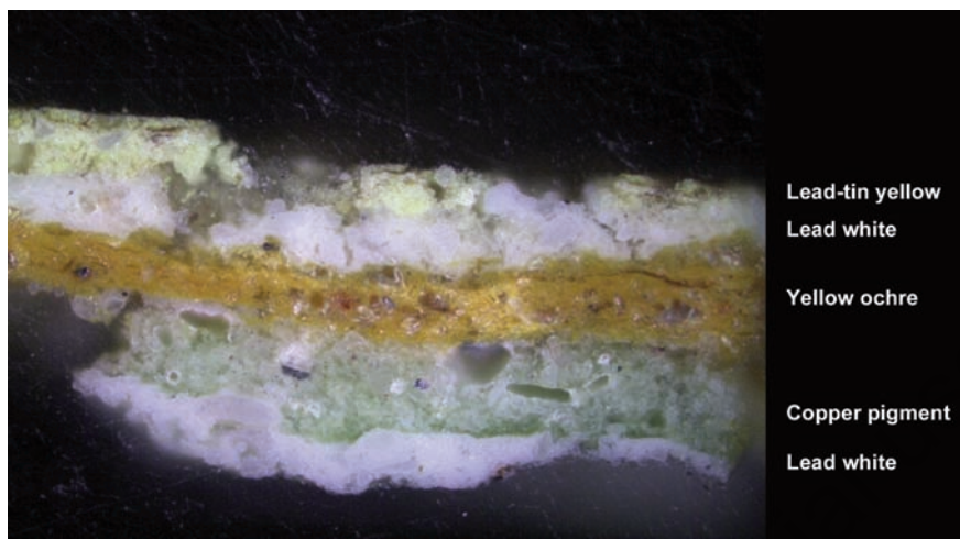
Figure 2. Stratigraphic section of a sample from a fragment of angel wing belonging to the archivolts (Bdx 14301). The green of the first coloured layer consists of a copper-based pigment, while the yellow-green of the upper layer is a repaint of lead-tin yellow (magnification x200). Reproduced with permission of S. Castandet, Centre de Recherche en Physique appliquée à l'Archéologie, Bordeaux, France.
