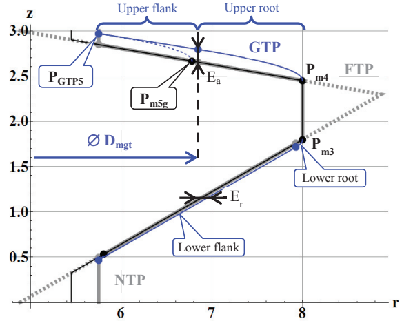
Fig. 4. Interference and errors - case B: D = 16 mm; P = 3 mm; D_m = 10 mm; \alpha_1 = 60^\circ ; \alpha_2 = 80^\circ .
