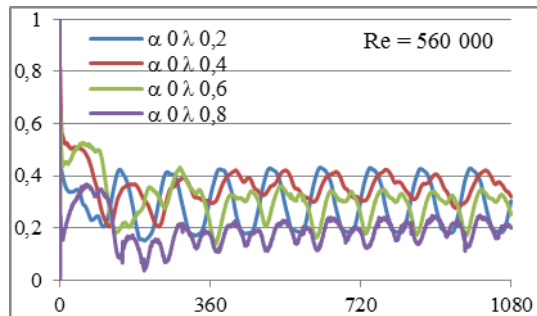
Fig. 21 Re=560\,000 , \alpha=0 degree
