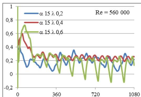
Fig. 23 Re=560\,000 , \alpha=15 degrees
