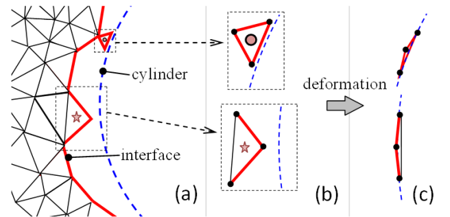
Figure 5. One kept triangle associating with 2 drilling interface edges (a,b) and the corresponding deformed version (c)
