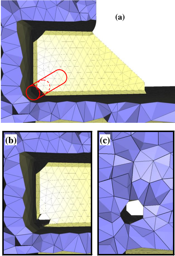
Figure 11 Insertion of a cylindrical hole into the 3D mesh of a caisson model (courtesy EDF-R&D).
