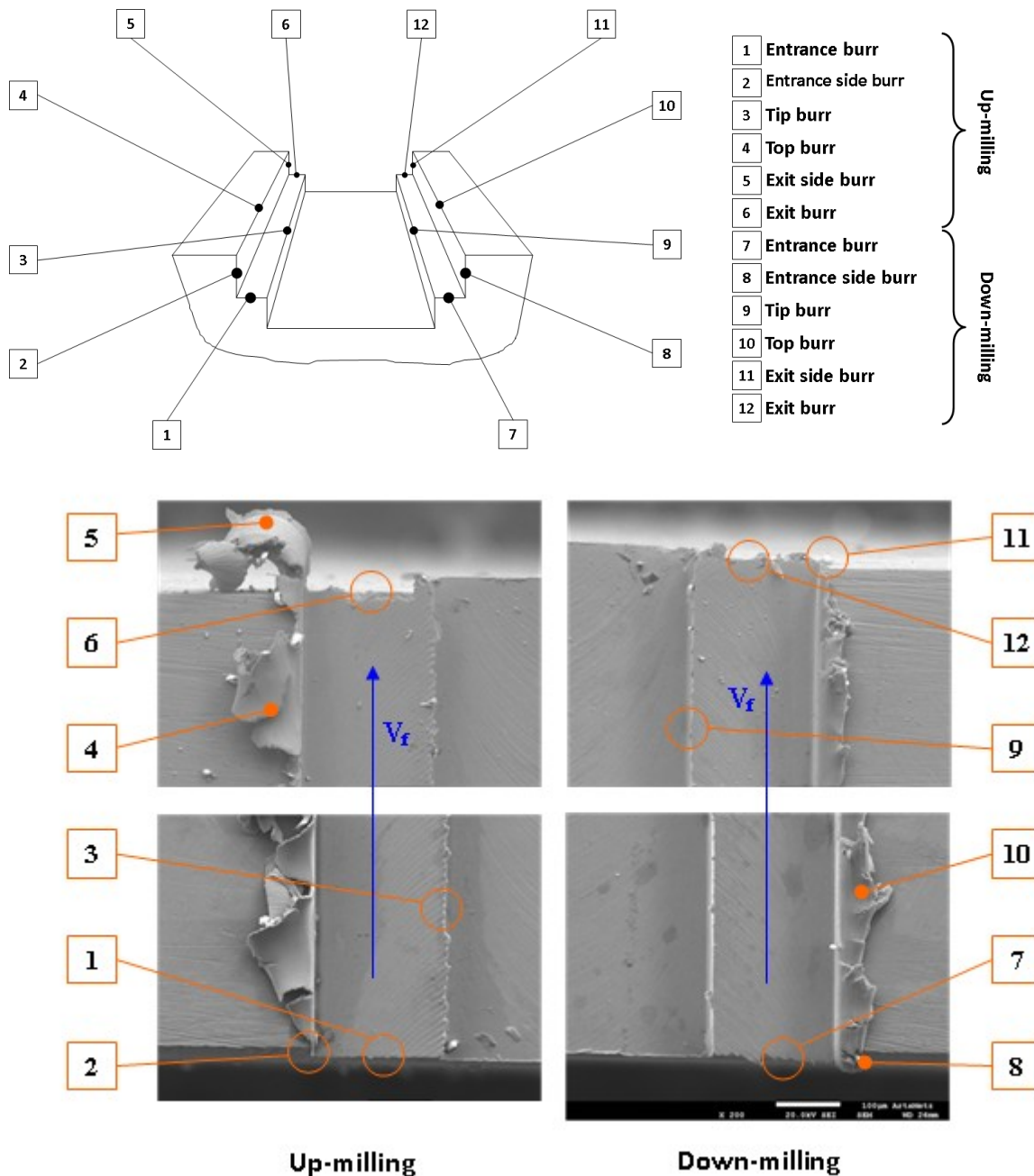
Fig. 5 : Entrance and exit of tests n°3 and n°4
