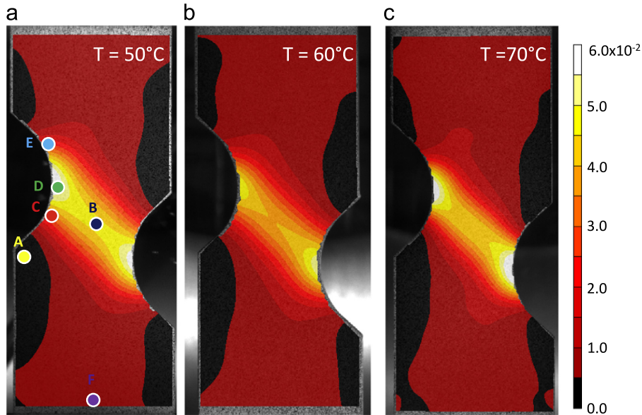
Fig. 2. Longitudinal strain fields measured by DIC for the three temperatures and the location of the six particular material points (a) \epsilon_{yy} for T = 50 °C, (b) \epsilon_{yy} for T = 60 °C, (c) \epsilon_{yy} for T = 70 °C.
