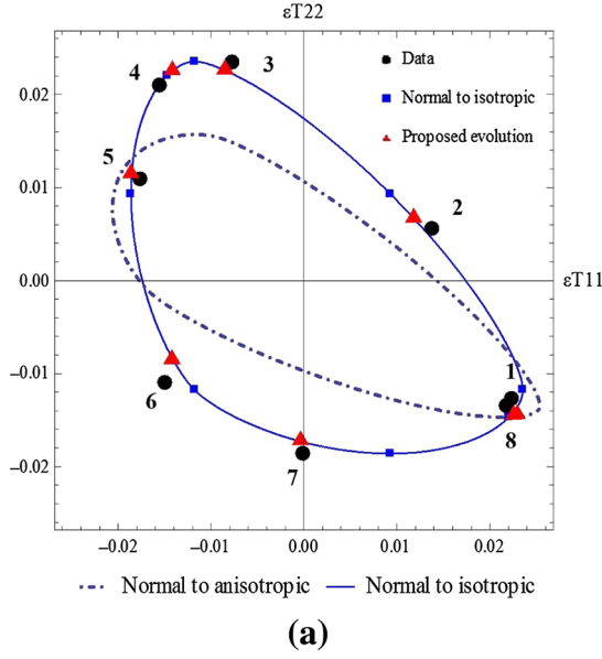
Fig. 6 Projection of the resulting transformation strains according to the proposed evolution law for the rolled (a) and the drawn specimen (b) for \xi = 70\% on the plane \epsilon_{11}^T - \epsilon_{22}^T
