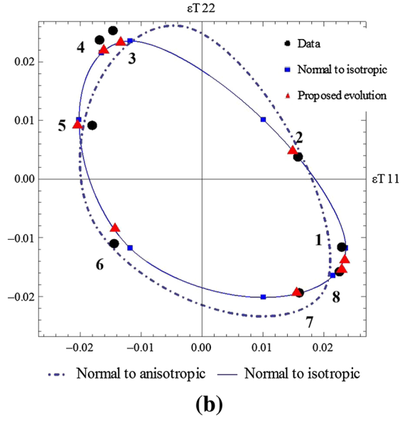
Fig. 6 Projection of the resulting transformation strains according to the proposed evolution law for the rolled (a) and the drawn specimen (b) for \xi = 70\% on the plane \epsilon_{11}^T - \epsilon_{22}^T
