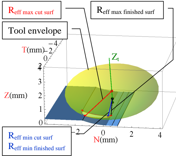
Fig. 1 Effective cutting radius on the cut and finished surface ( \beta_f = 20^\circ , \beta_n = 0^\circ , a_r = 0.4 mm, a_a = 0.3 mm)
